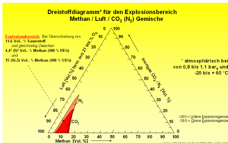
Figure 2 – Explosion limit of gas mixtures: Methane/Air/ CO 2 and Methane/Air/ N 2 ; concentrations are indicated in percent by volume in relation to the overall gas mixture; 15 % by vol. CH 4 / explosion limit, i.e. 5 % CH 4 = 100 % LEL (Own drawing based on BAM – Sicherheitstechnische Kenngrößen, ISBN 3-89701-746-6)
