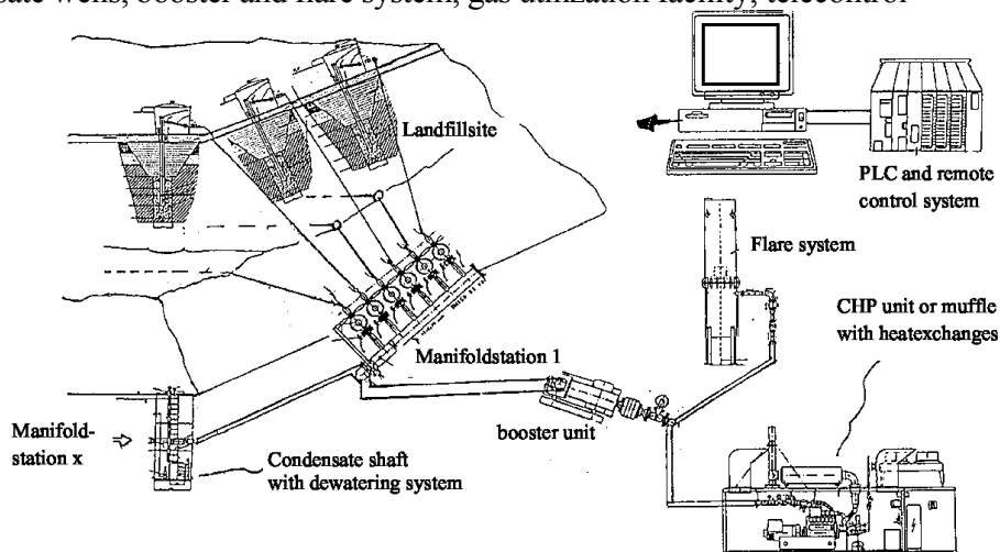
Figure 1 - Landfill gas extraction system (wellheads, manifold station, dewatering system, condensate wells, booster and flare system, gas utilization facility, telecontrol
